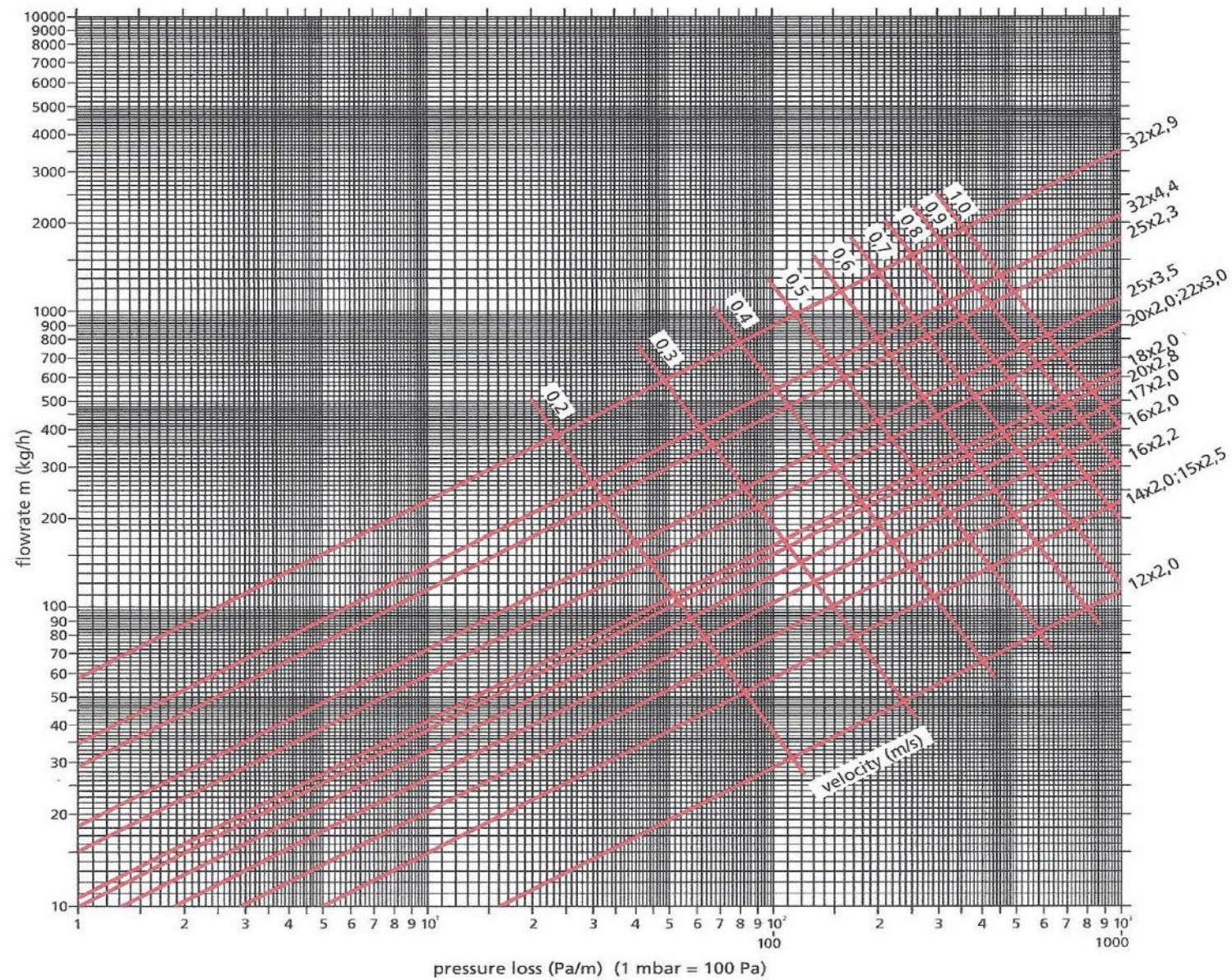
Drukverlies diagram Tubes International BV PE-RT Buis
